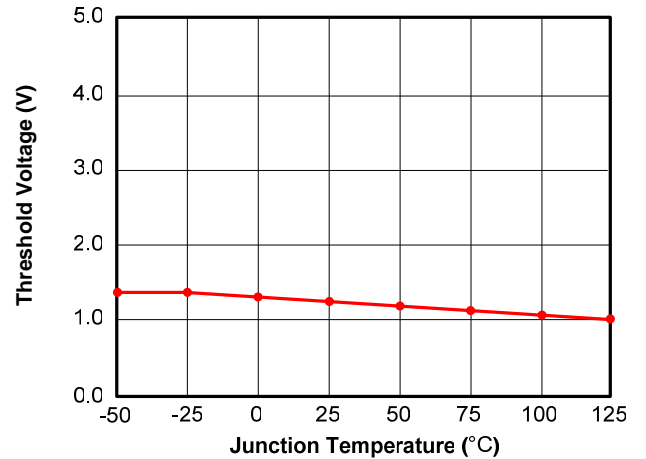
ON/OFF Threshold Voltage
